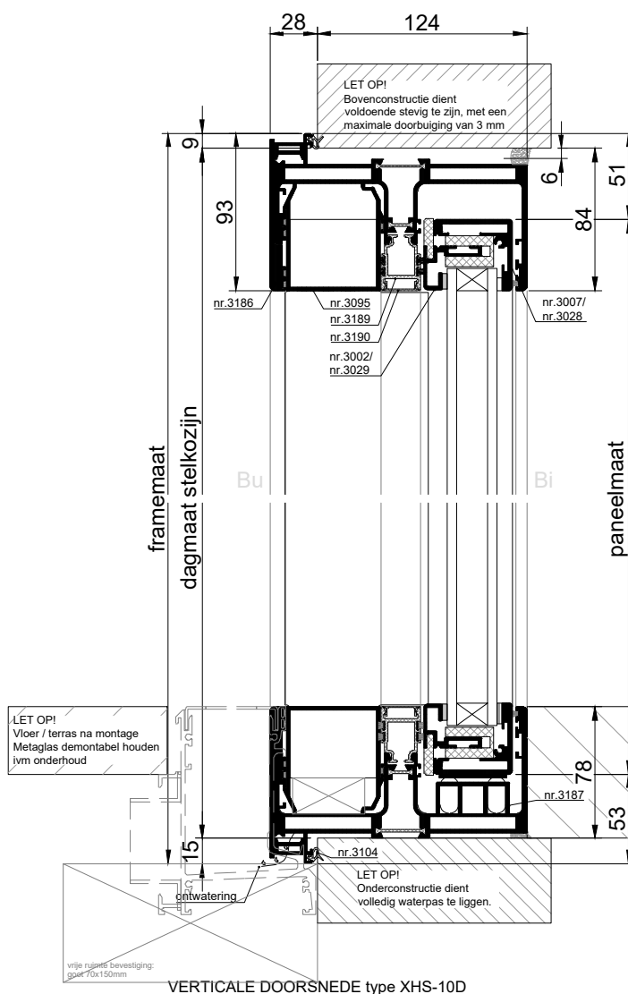
VERTICALE DOORSNEDE type XHS-10D
