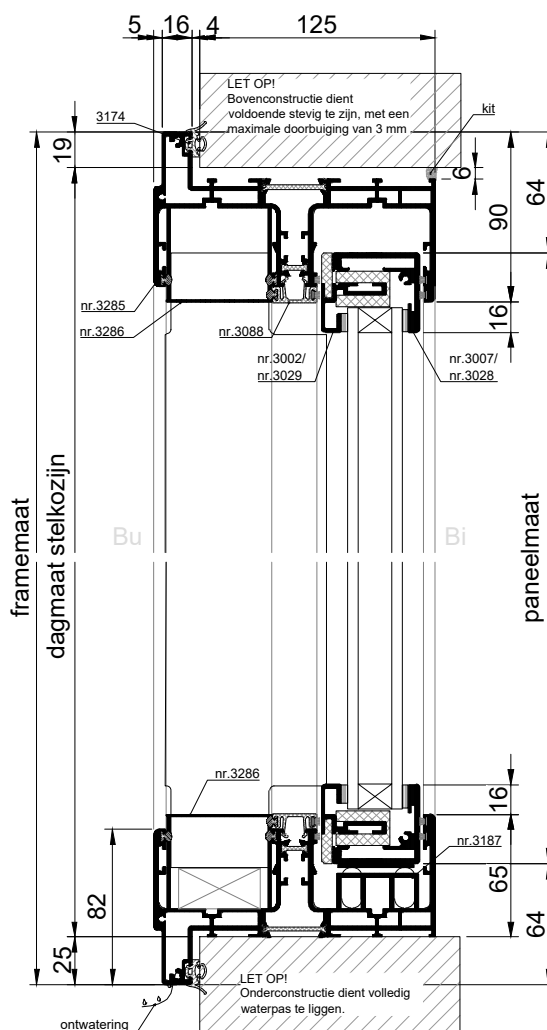
VERTICALE DOORSNEDE type XHS-17D
