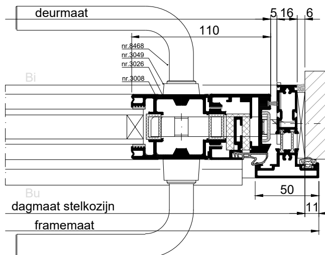
HORIZONTALE DOORSNEDE type XID-1A/E
