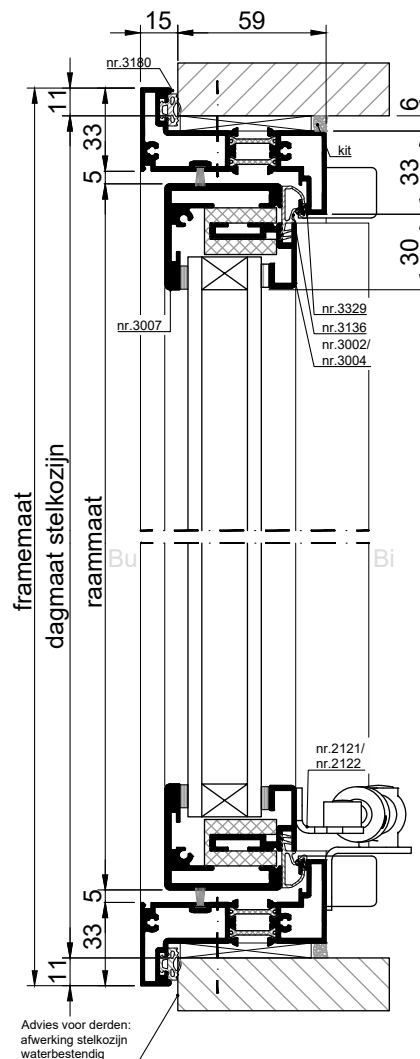
VERTICALE DOORSNEDE type XSU-1
