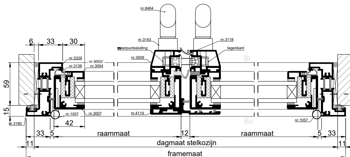
HORizontale DOORSNEDE type XSU-1
