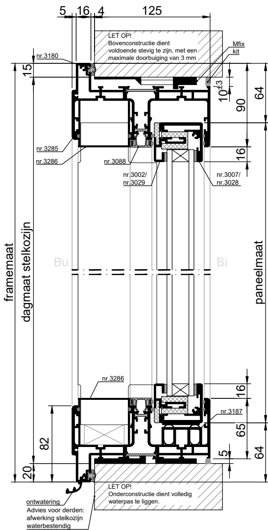
VERTICALE DOORSNEDE type XHS-17D
