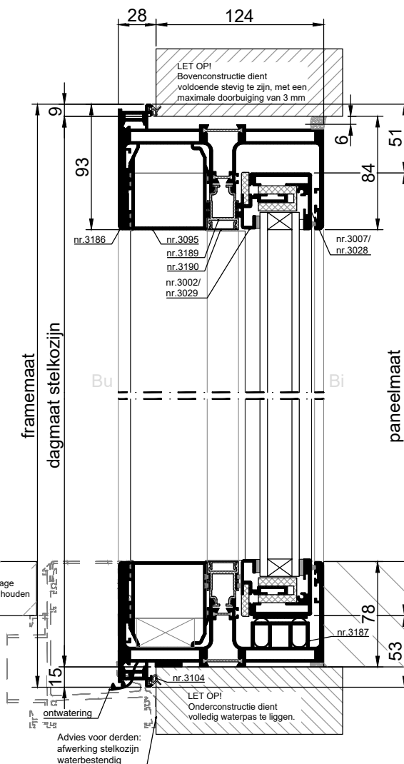
VERTICALE DOORSNEDE type XHS-10D
