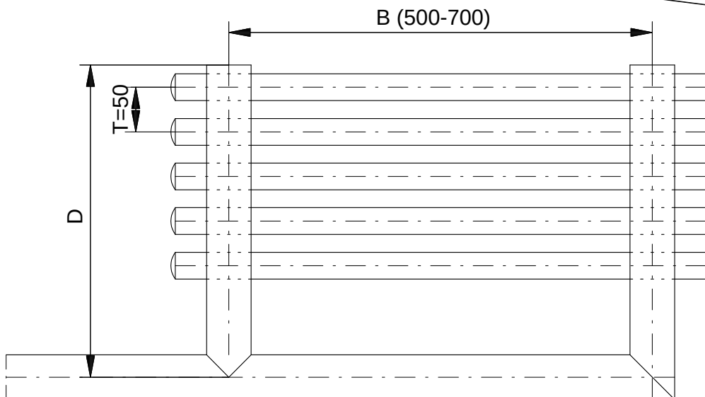
Rangeerstation nr. 8282 Model P (parallel parkeren) D = \text{aantal panelen} \times T + 100 \text{ mm} T = 50 \text{ mm}
