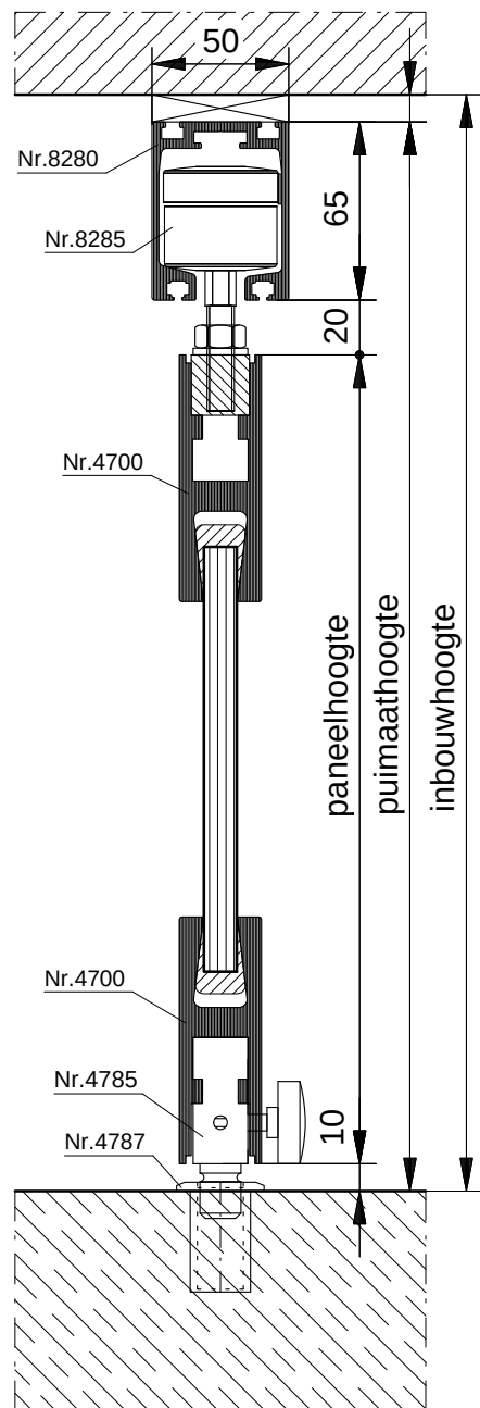
VERTICALE DOORSNEDE HSW-4A
