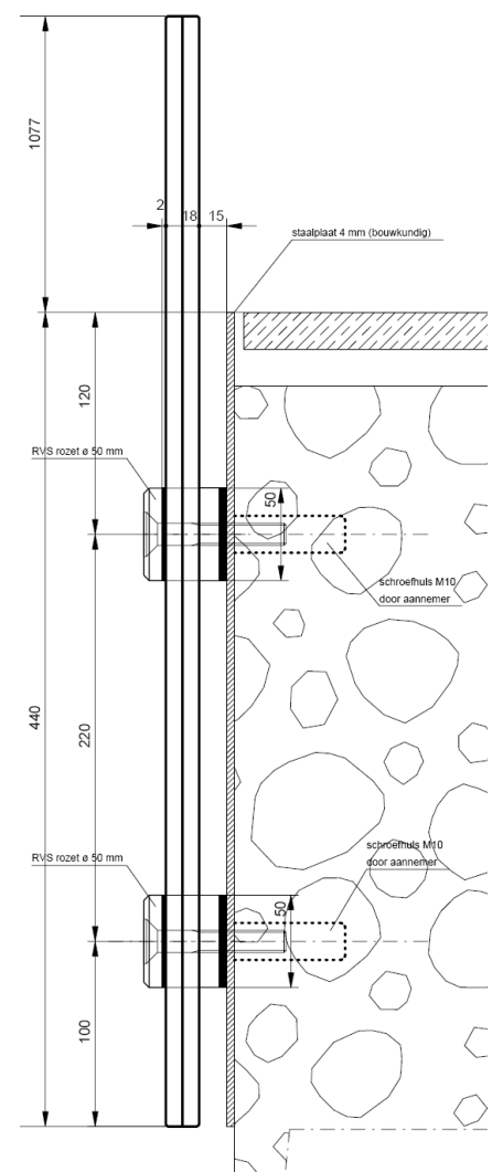
Verticale doorsnede type BW-4
