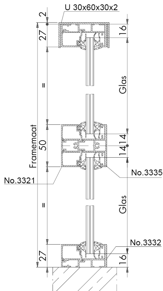
Verticale doorsnede type BW-1
