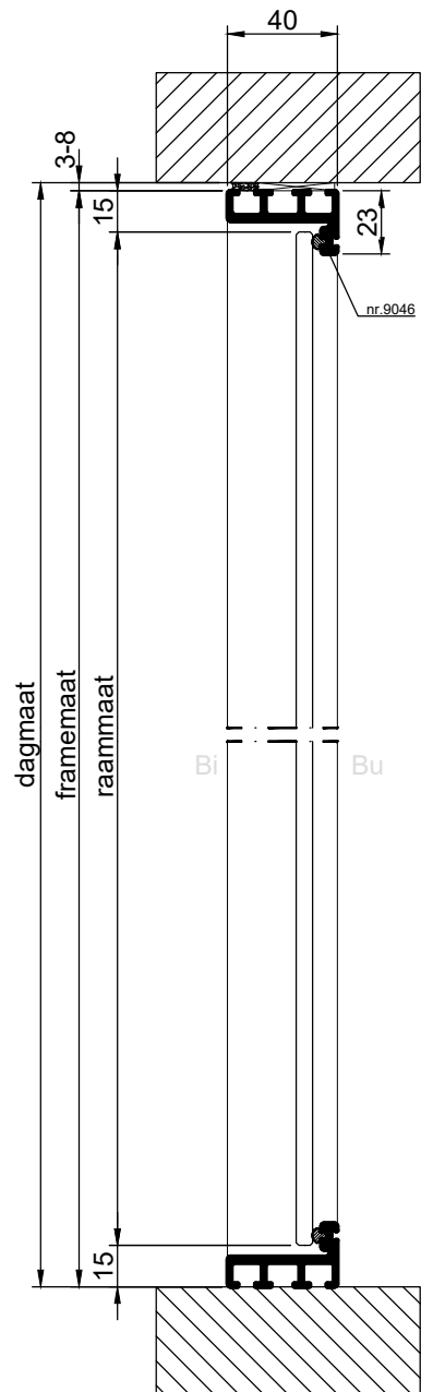
VERTICALE DOORSNEDE type DVR-7
